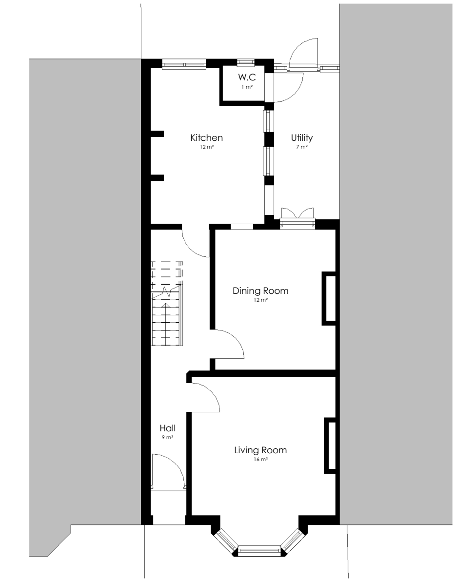
Existing Ground Floor 1 : 100
