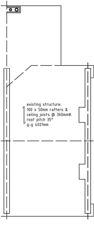
ROOF PLAN
