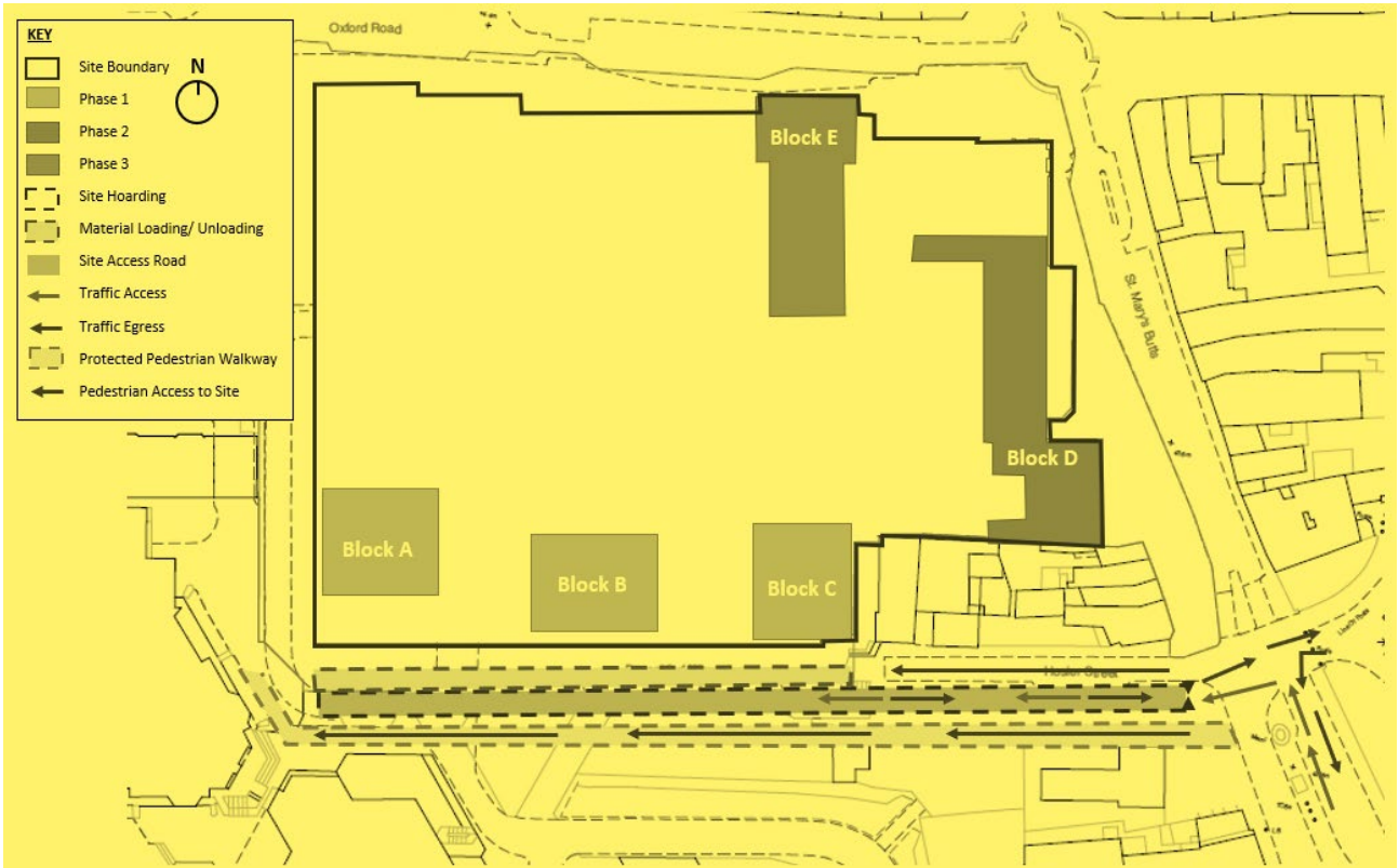
Figure 5.5 Site Establishment and Logistics Layout Plan
