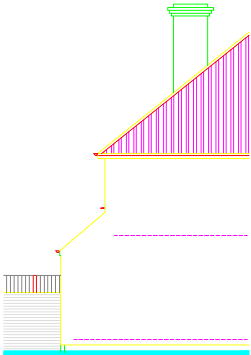
Side Elevation
