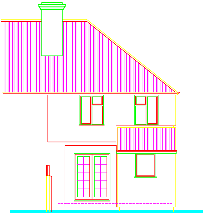
Rear Elevation
