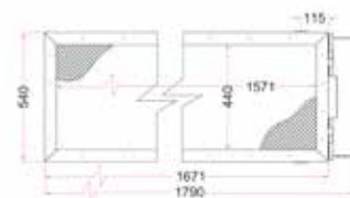
Air Discharge View
