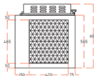
Air Intake View
