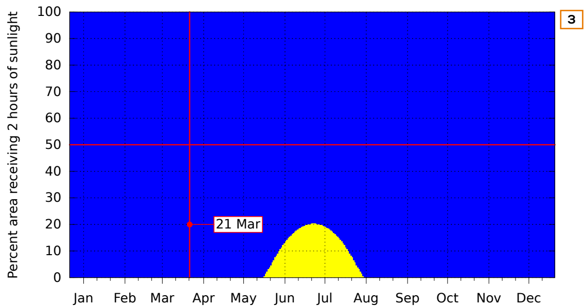
Fig. 50: Sun Hours on Ground - Annual BRE Compliance diagram - Area 3
