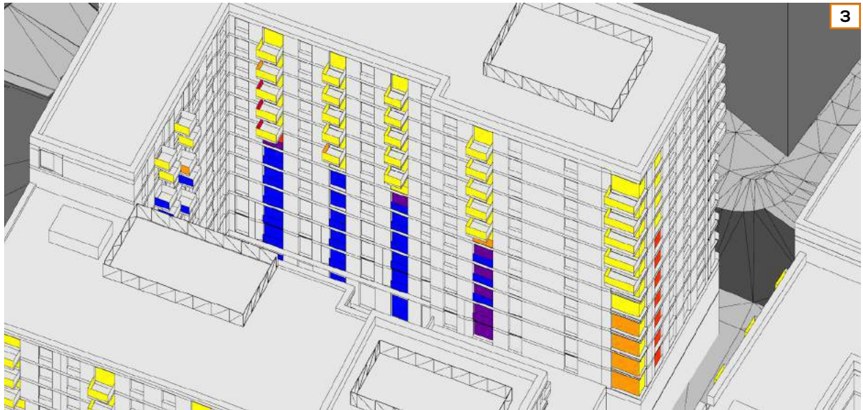
Fig. 43: Winter Probable Sunlight Hours - View 3
