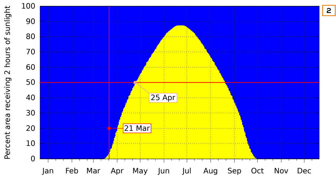
Fig. 49: Sun Hours on Ground - Annual BRE Compliance diagram - Area 2
