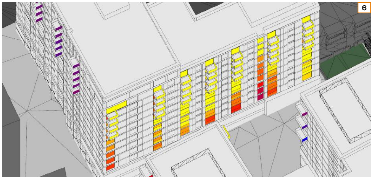
Fig. 46: Annual Probable Sunlight Hours - View 6
