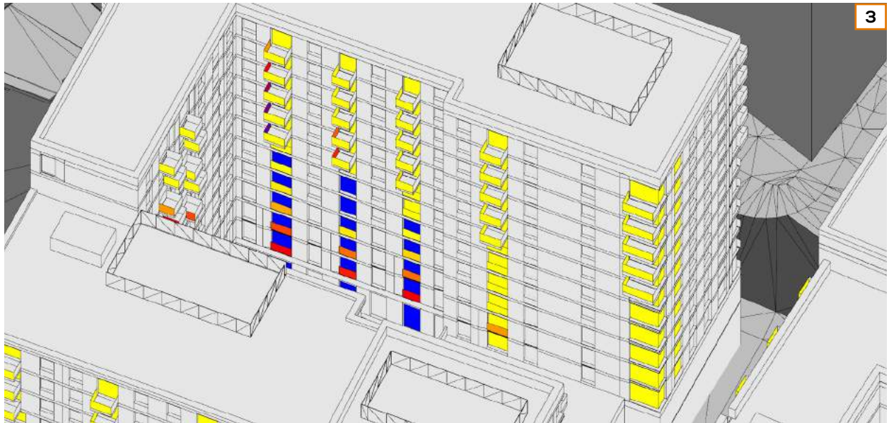
Fig. 41: Annual Probable Sunlight Hours - View 3
