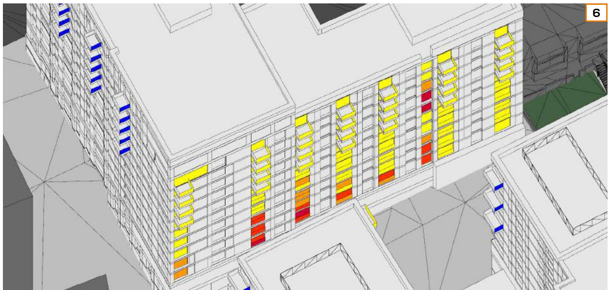
Fig. 48: Winter Probable Sunlight Hours - View 6
