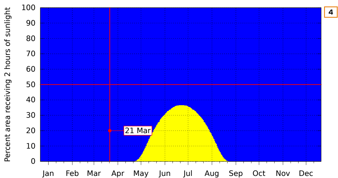
Fig. 51: Sun Hours on Ground - Annual BRE Compliance diagram - Area 4
