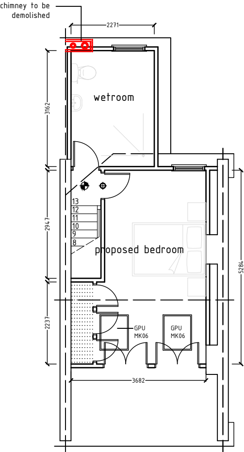
ROOF PLAN
