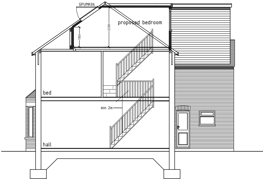
SECTION THRO.
