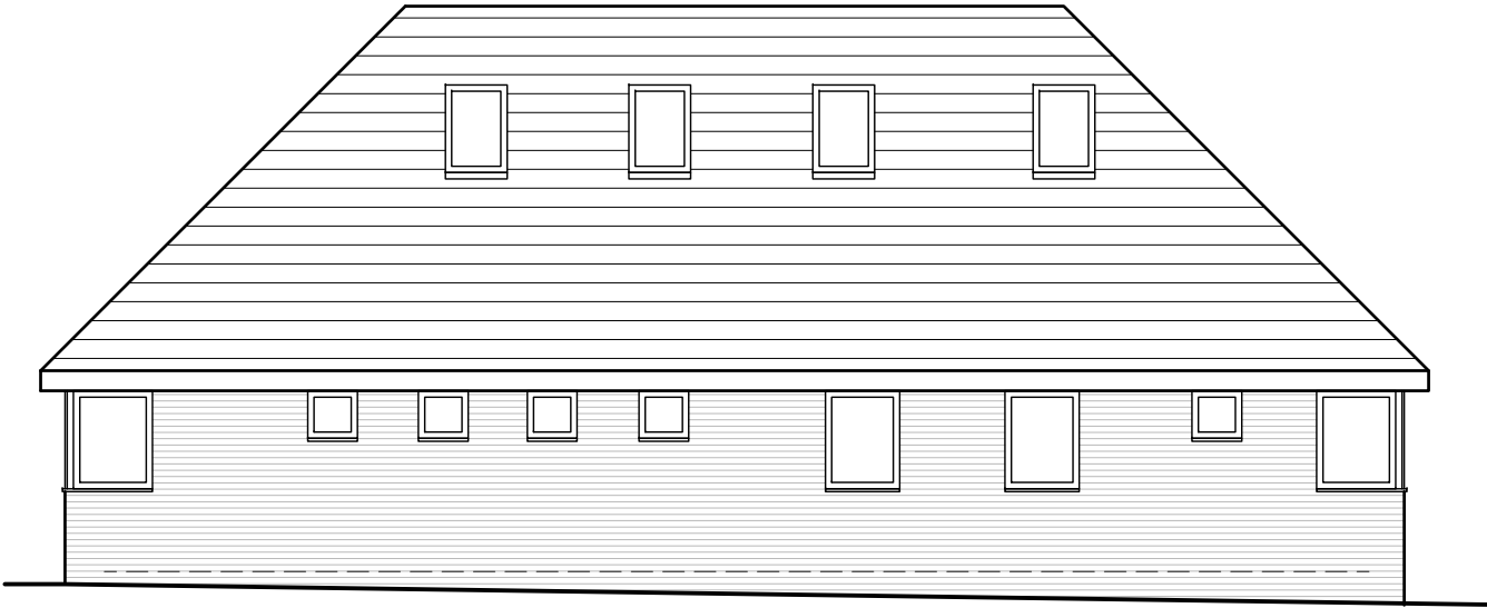
Rear Elevation (to North)
