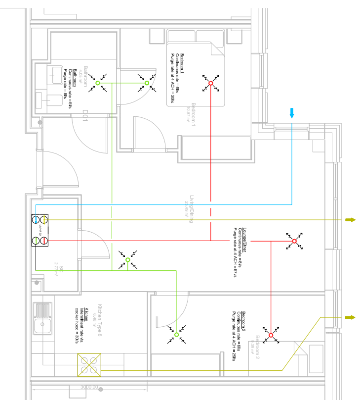
APARTMENT TYPE 2B
