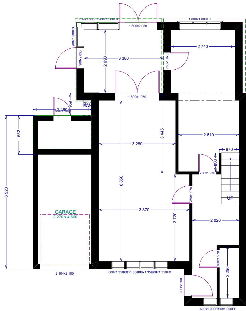
Ground Floor Plan | Existing 1:100@A3
