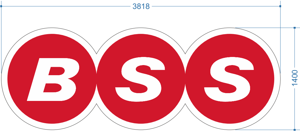
ITEM C | x 1 Aluminium tray with 25mm deep returns finished White with applied Red S/A vinyls to face. Illuminated via overhead trough light.
