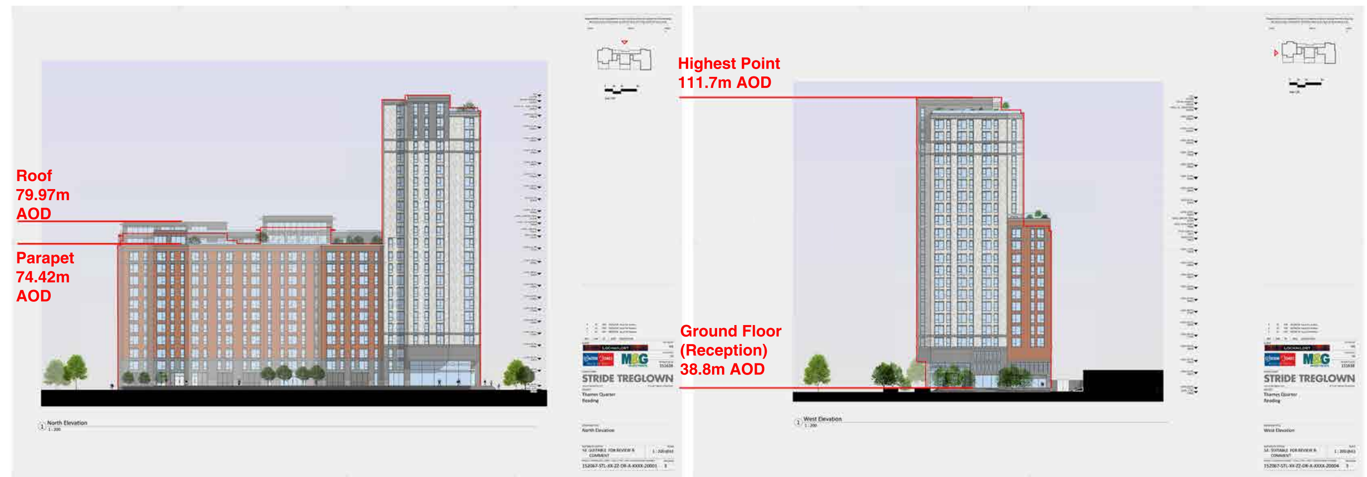
Proposed North Elevation no 152067-STL-XX-ZZ-DR-A-XXXX-20001 Rev 3
