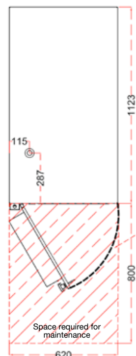
Top View
