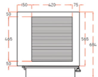
Air Discharge View
