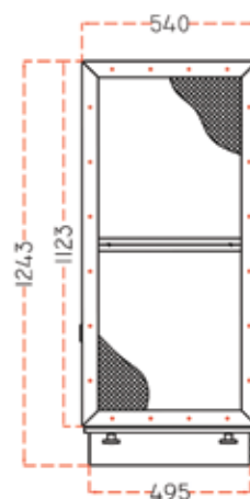
Air Intake View
