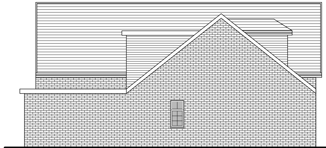
PROPOSED SIDE ELEVATION (FROM NO. 174) SCALE 1/100
