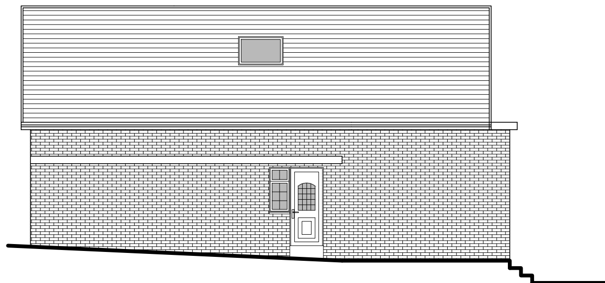
PROPOSED SIDE ELEVATION (FROM NO. 170) SCALE 1/100
