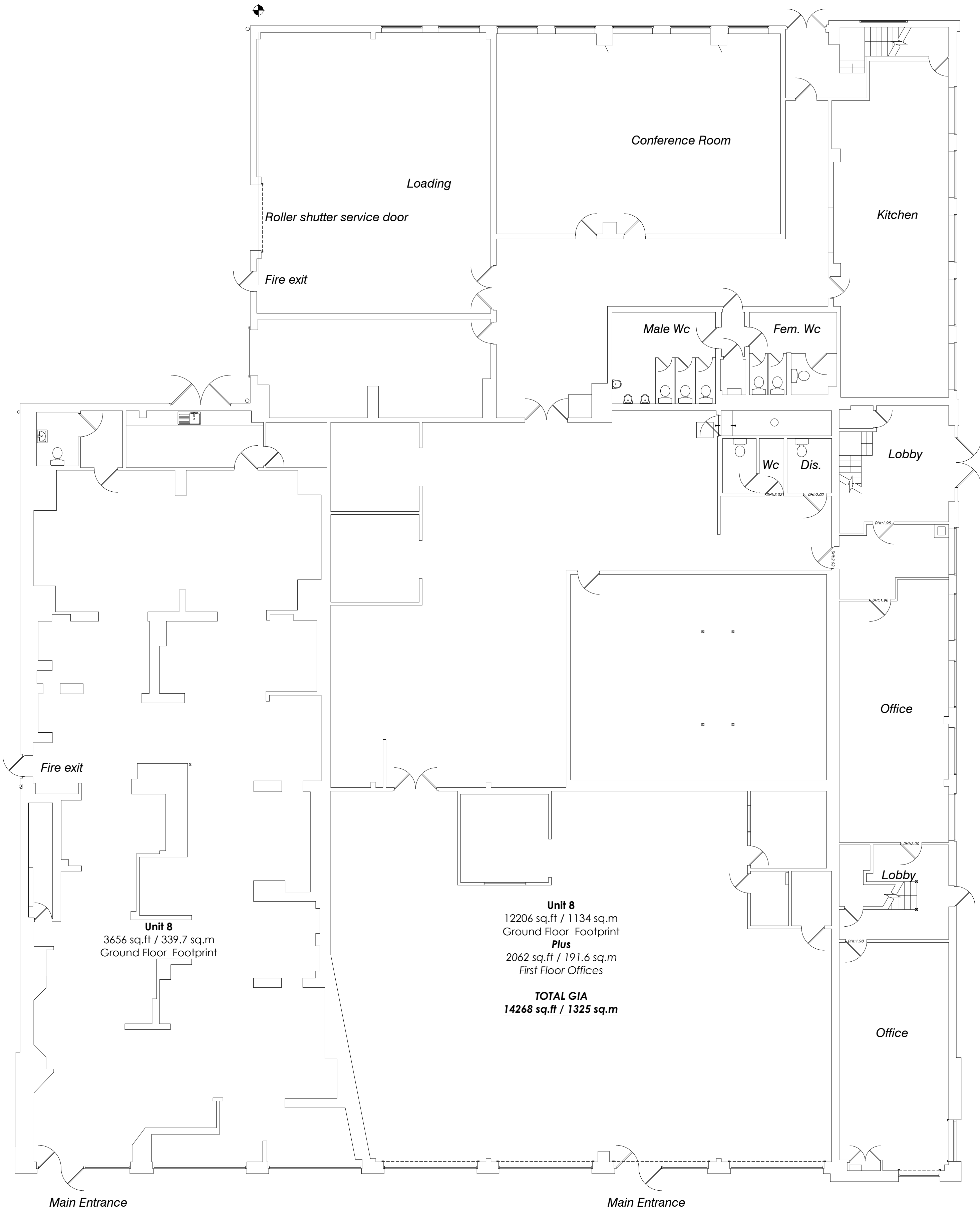
Existing Ground Floor GA Plan
