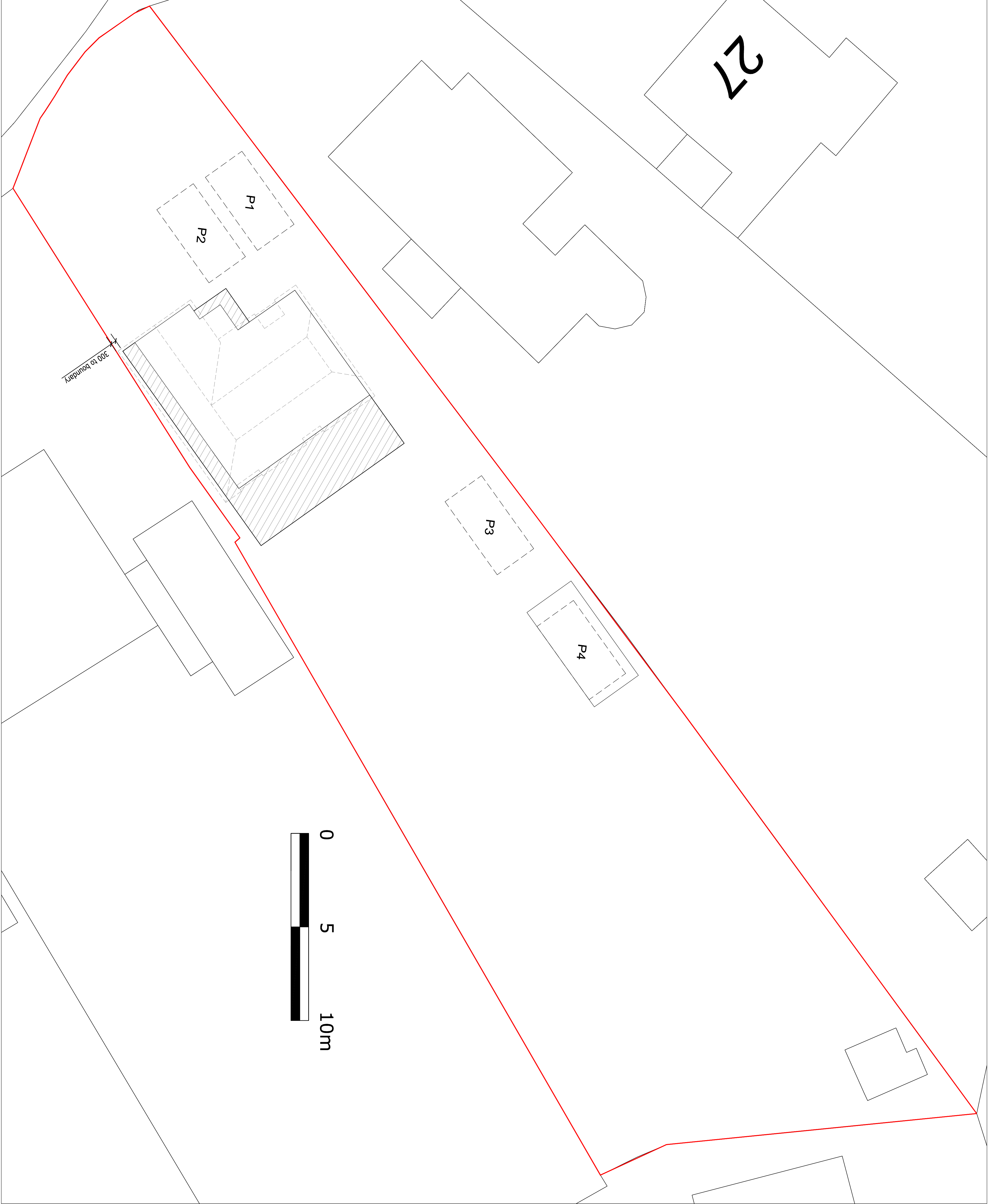
Block Plan (1:100)
