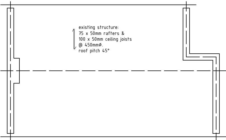
ROOF PLAN
