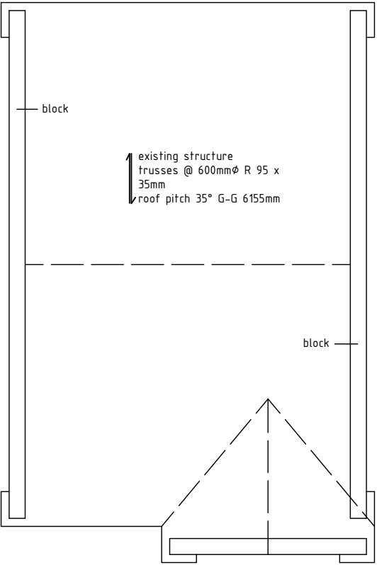
ROOF PLAN
