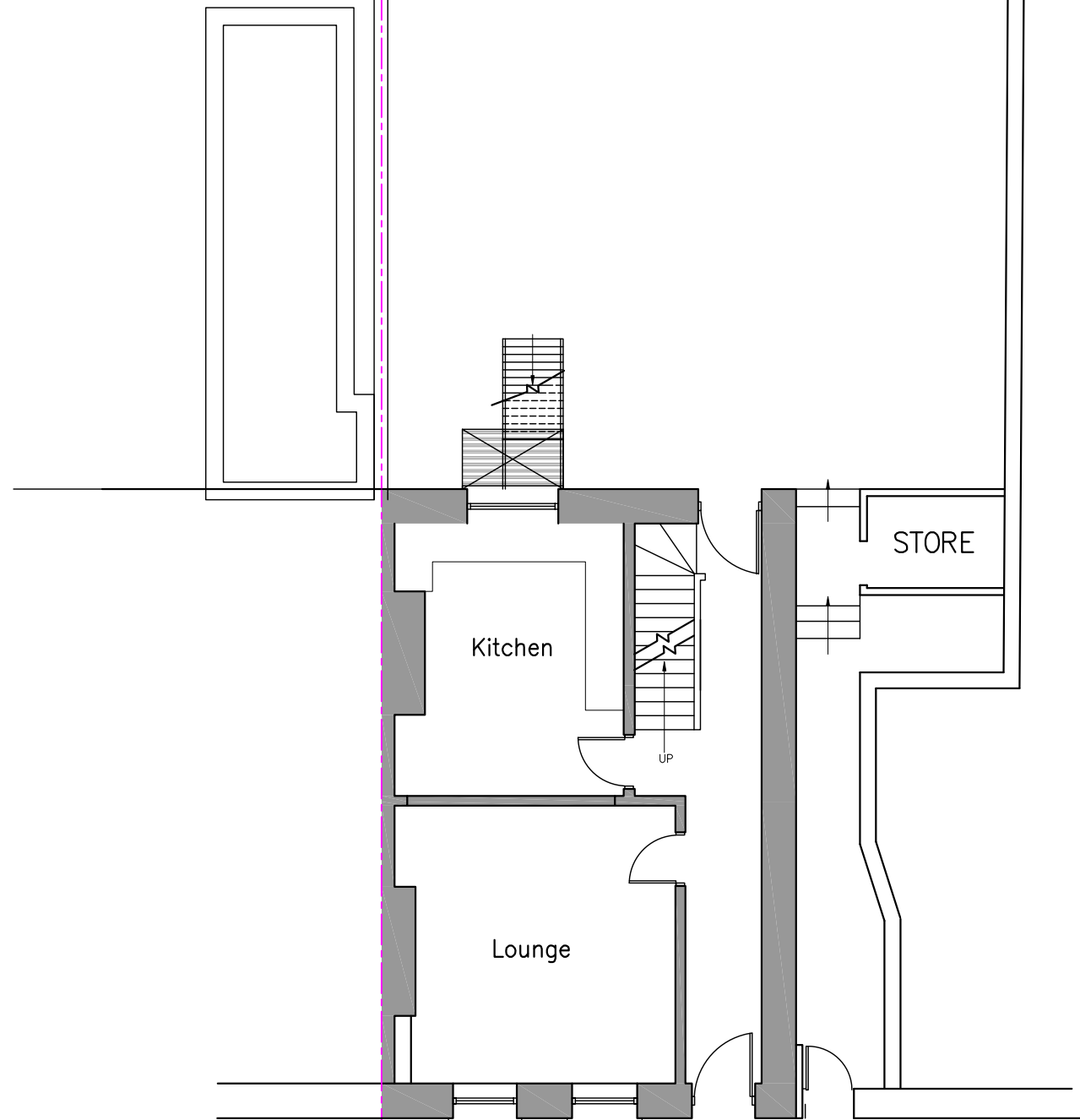
UPPER GROUND FLOOR SCALE 1:100
