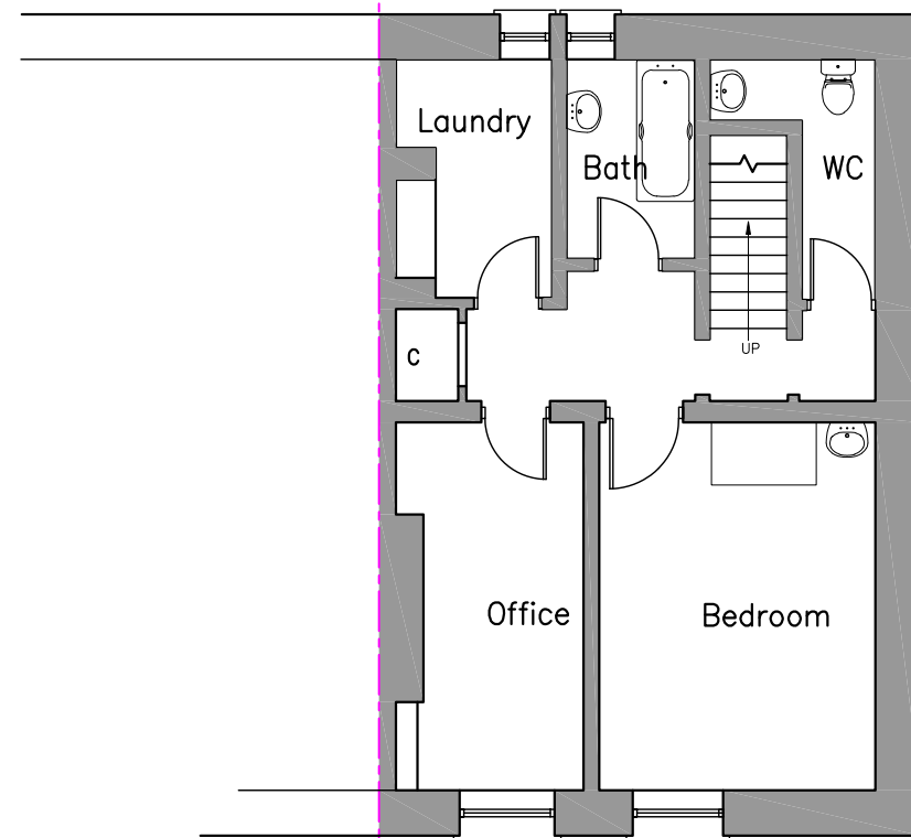
LOWER GROUND FLOOR SCALE 1:100
