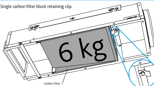
Figure 8. Single carbon filter block removal.
