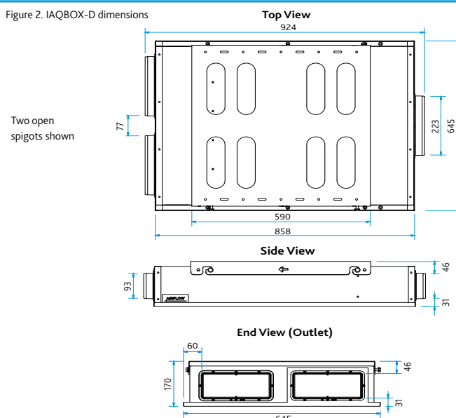
Figure 2. IAQBOX-D dimensions
