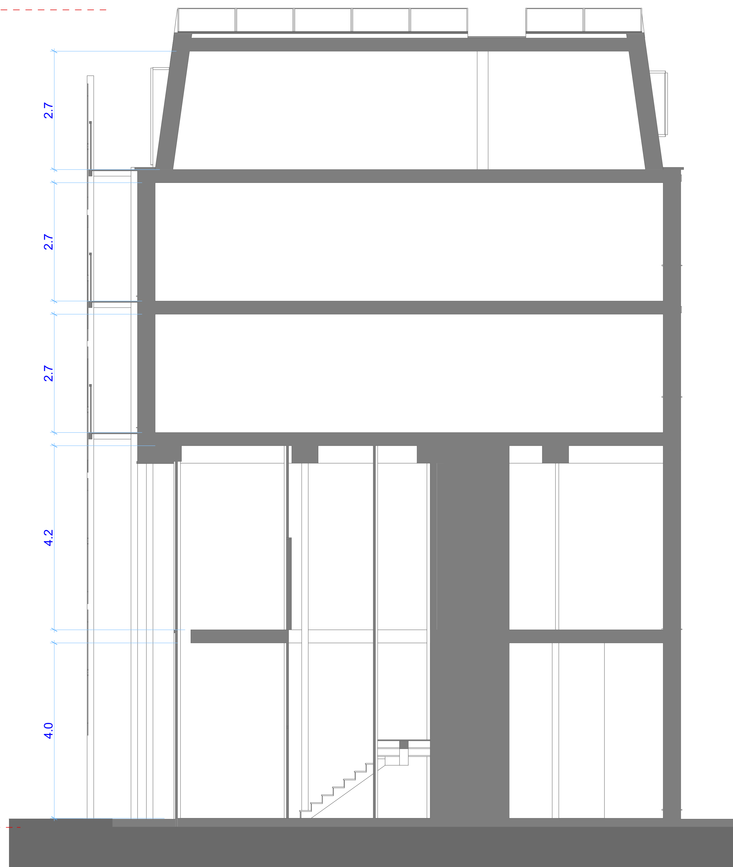
Section A-A Proposed 1:50
