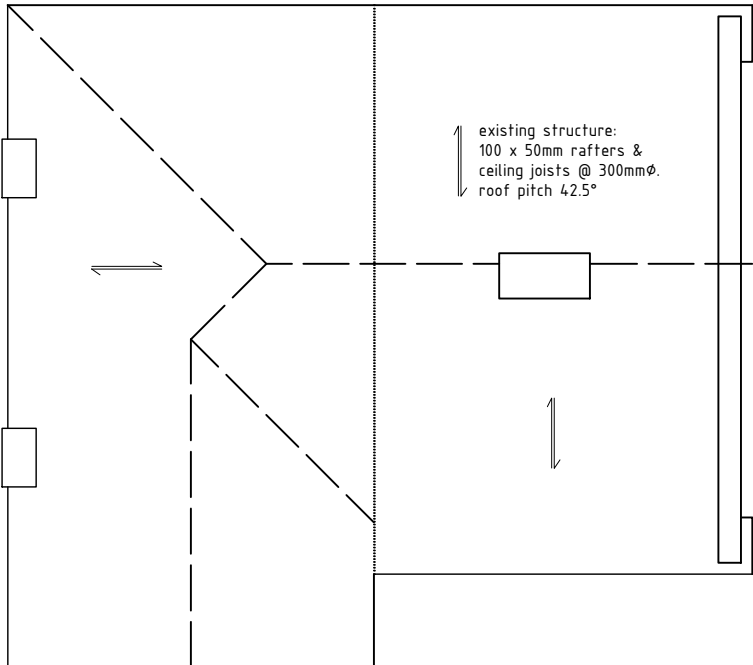
ROOF PLAN
