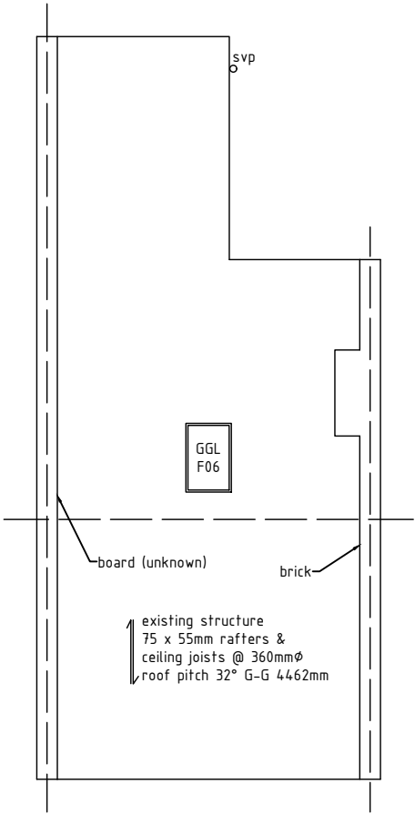
ROOF PLAN
