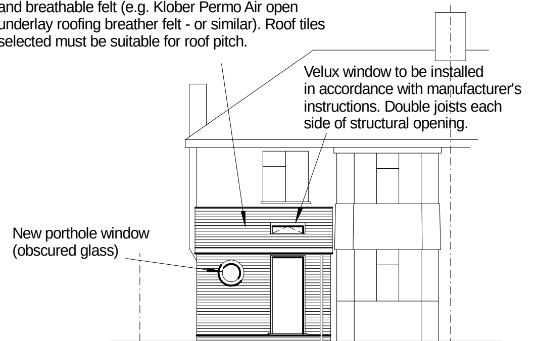
FRONT
