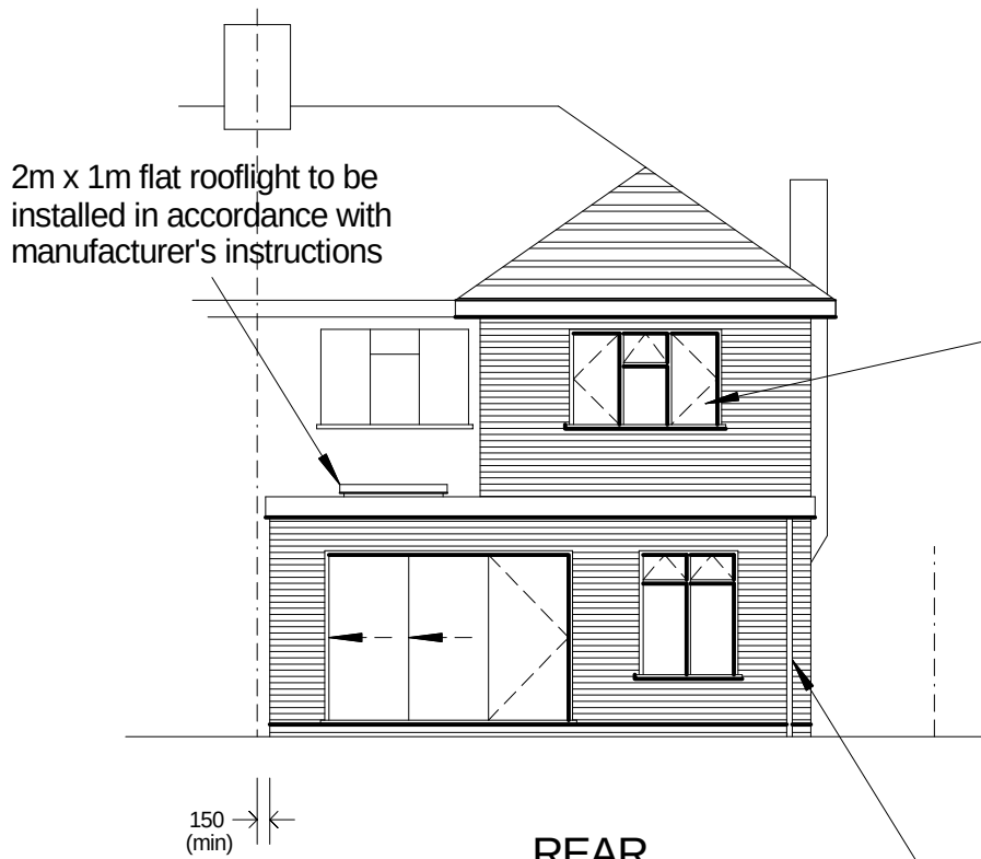
REAR
