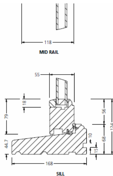
SILL
