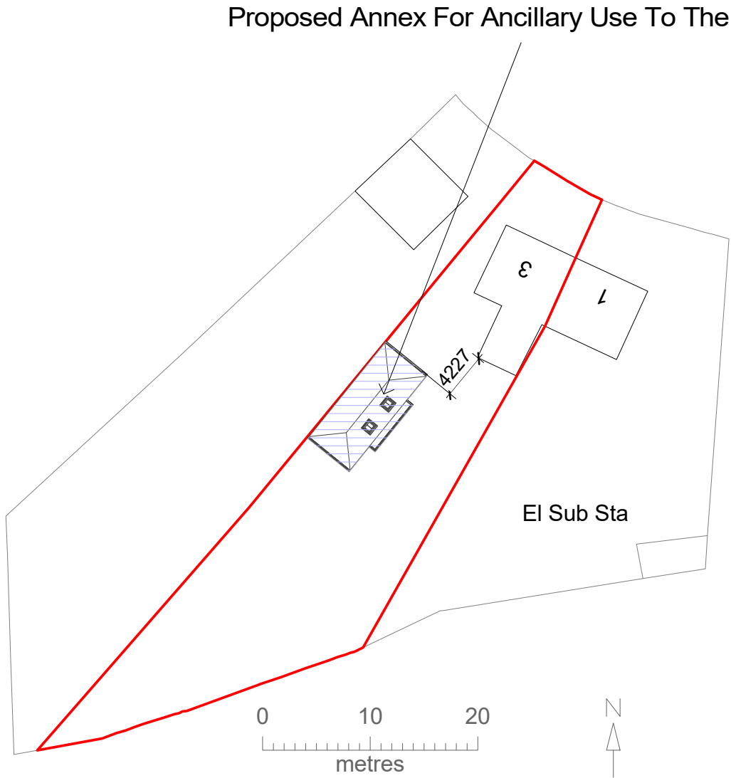
1 500 Proposed Site Plan 1 : 500
