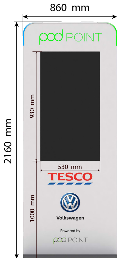
FRONT ELEVATION MEDIA CHARGER WITH LCD SCREEN
