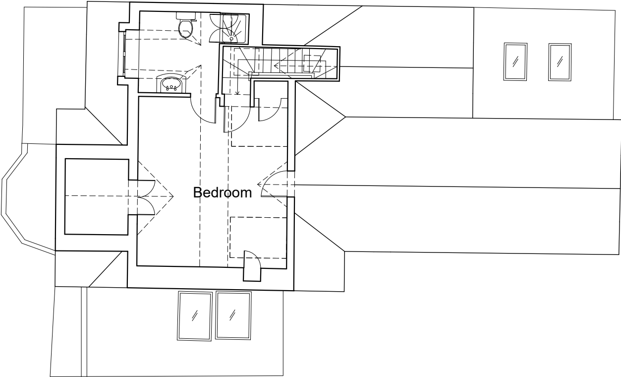
1 Existing Second Floor plan
