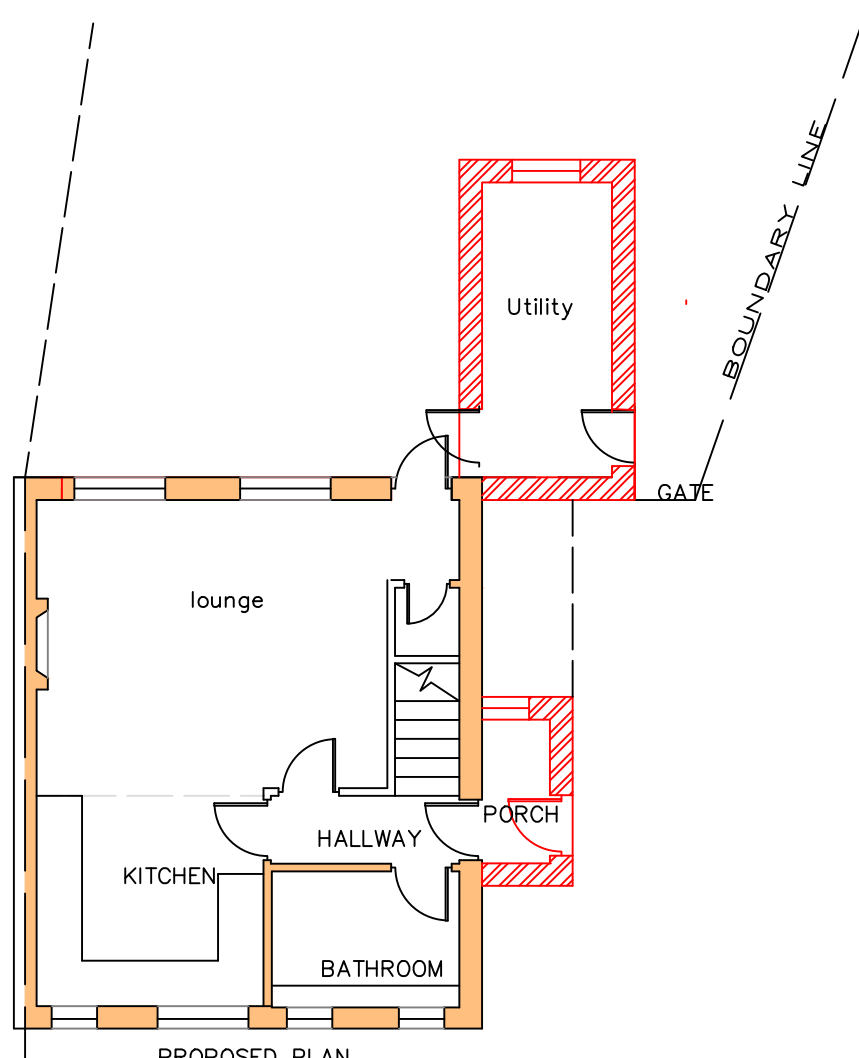
PROPOSED PLAN
