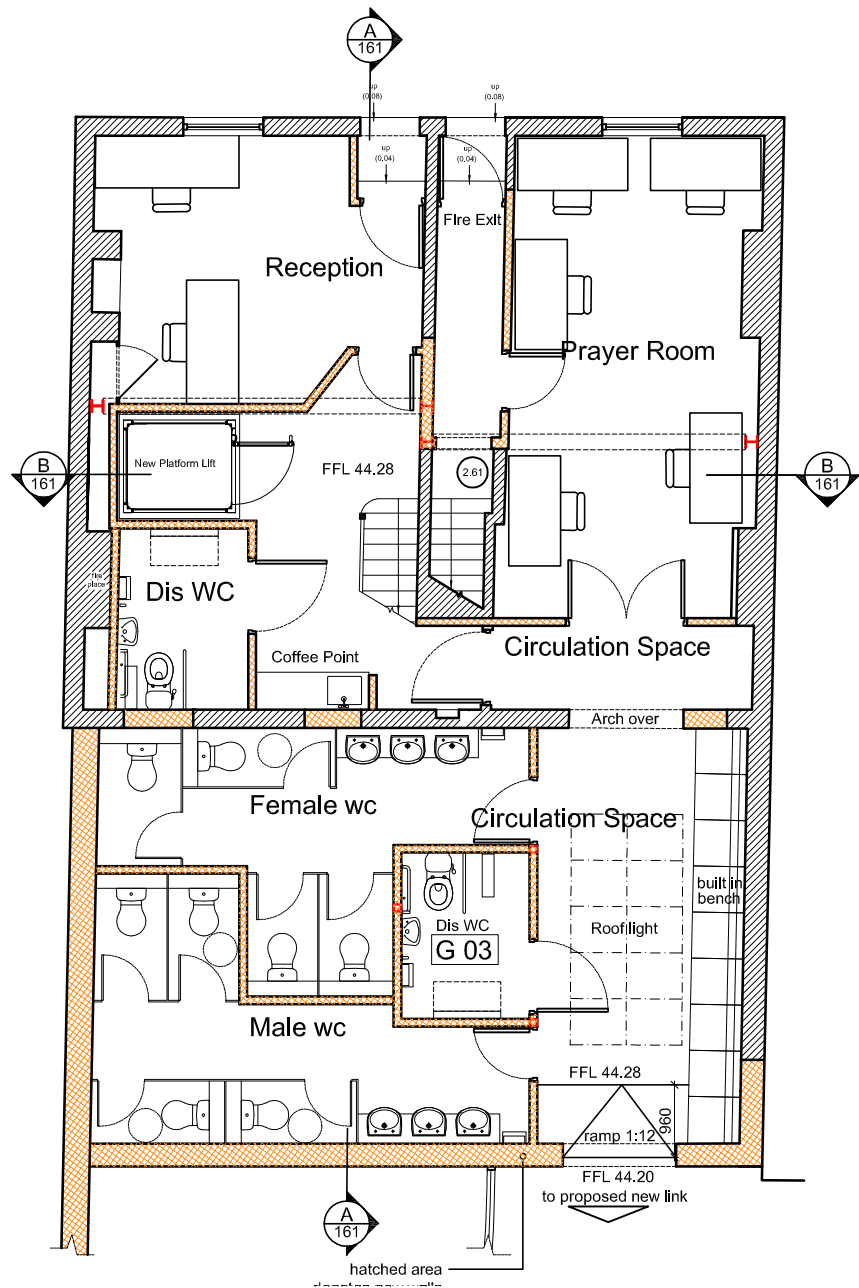
1 Ground Floor Plan Scale: 1:100
