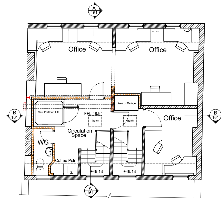
3 Second Floor Plan Scale: 1:100
