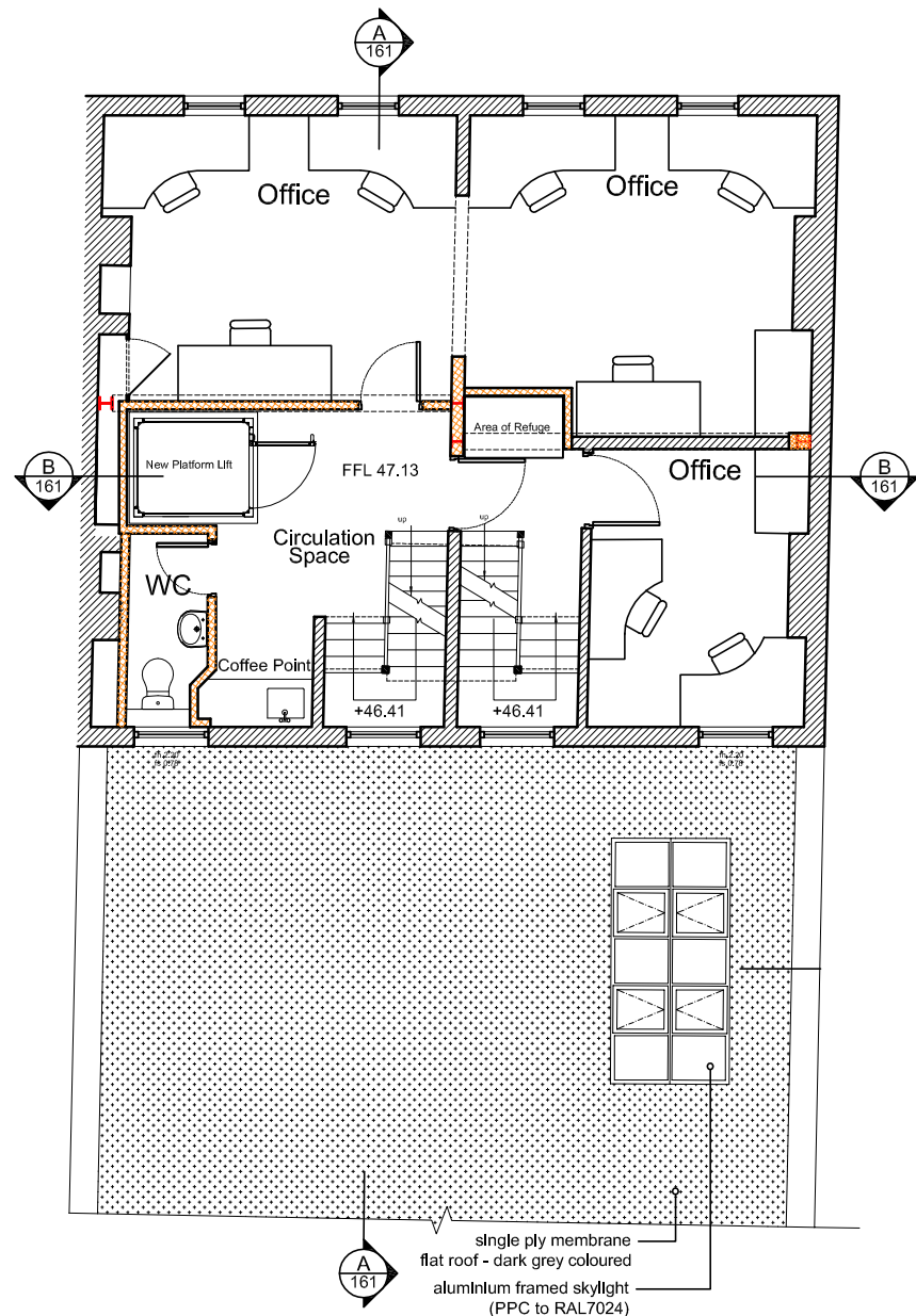
2 First Floor Plan Scale: 1:100
