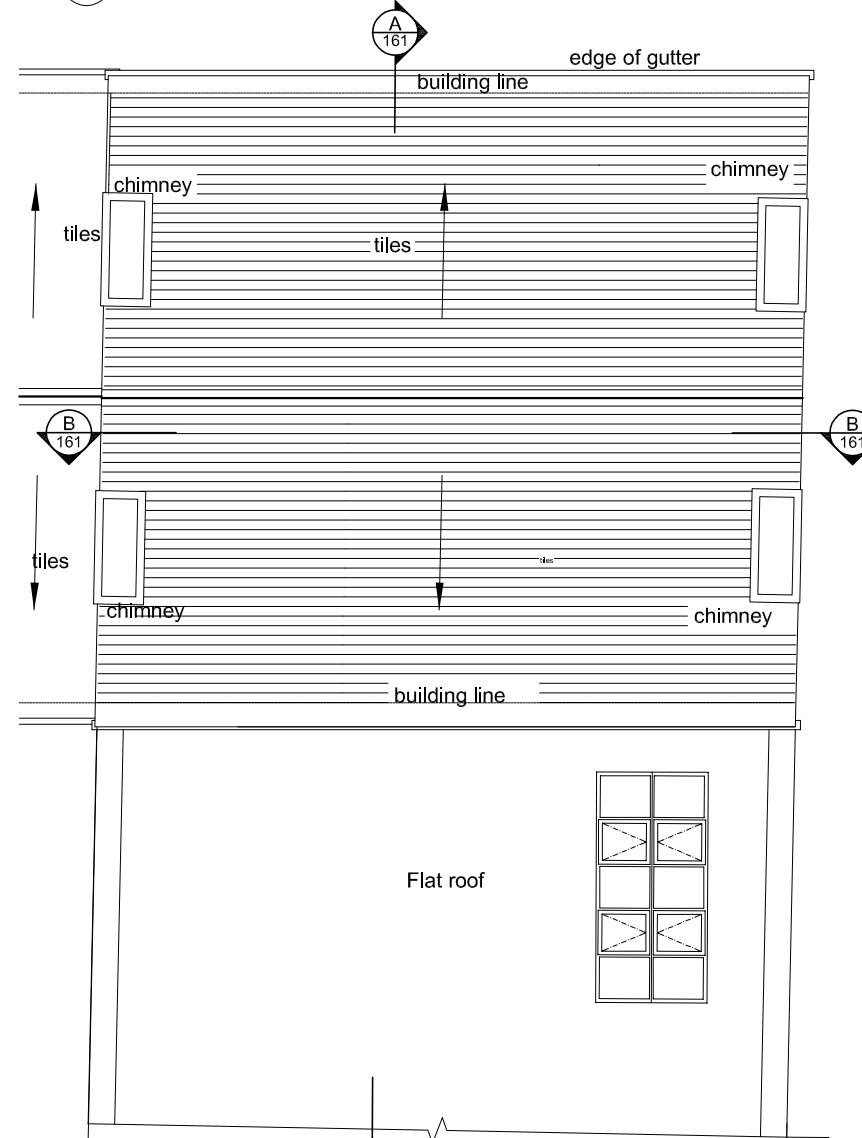
4 Roof Plan Scale: 1:100
