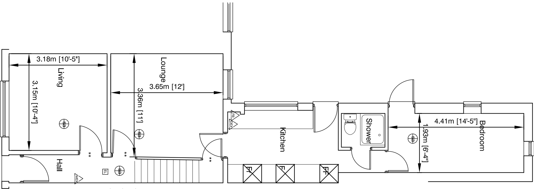
front Ground Floor Plan
