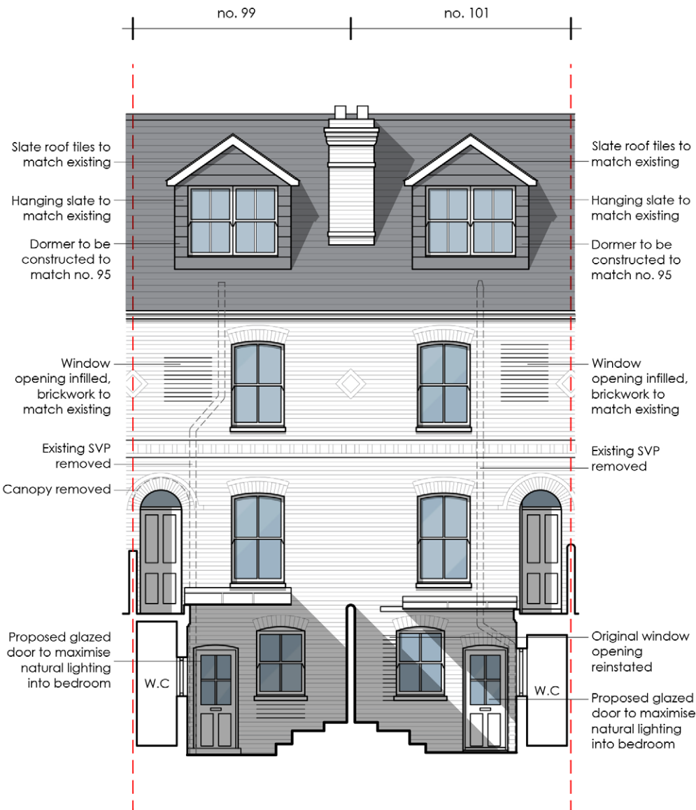
PROPOSED SOUTH (FRONT) ELEVATION 1:100
