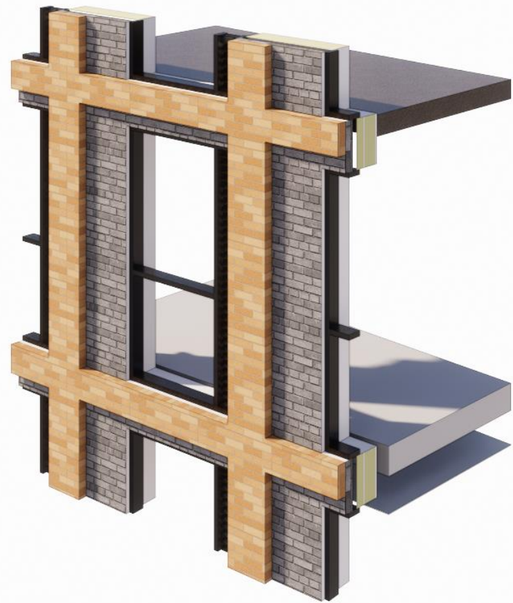
FAÇADE TYPE 3 - Brickwork
