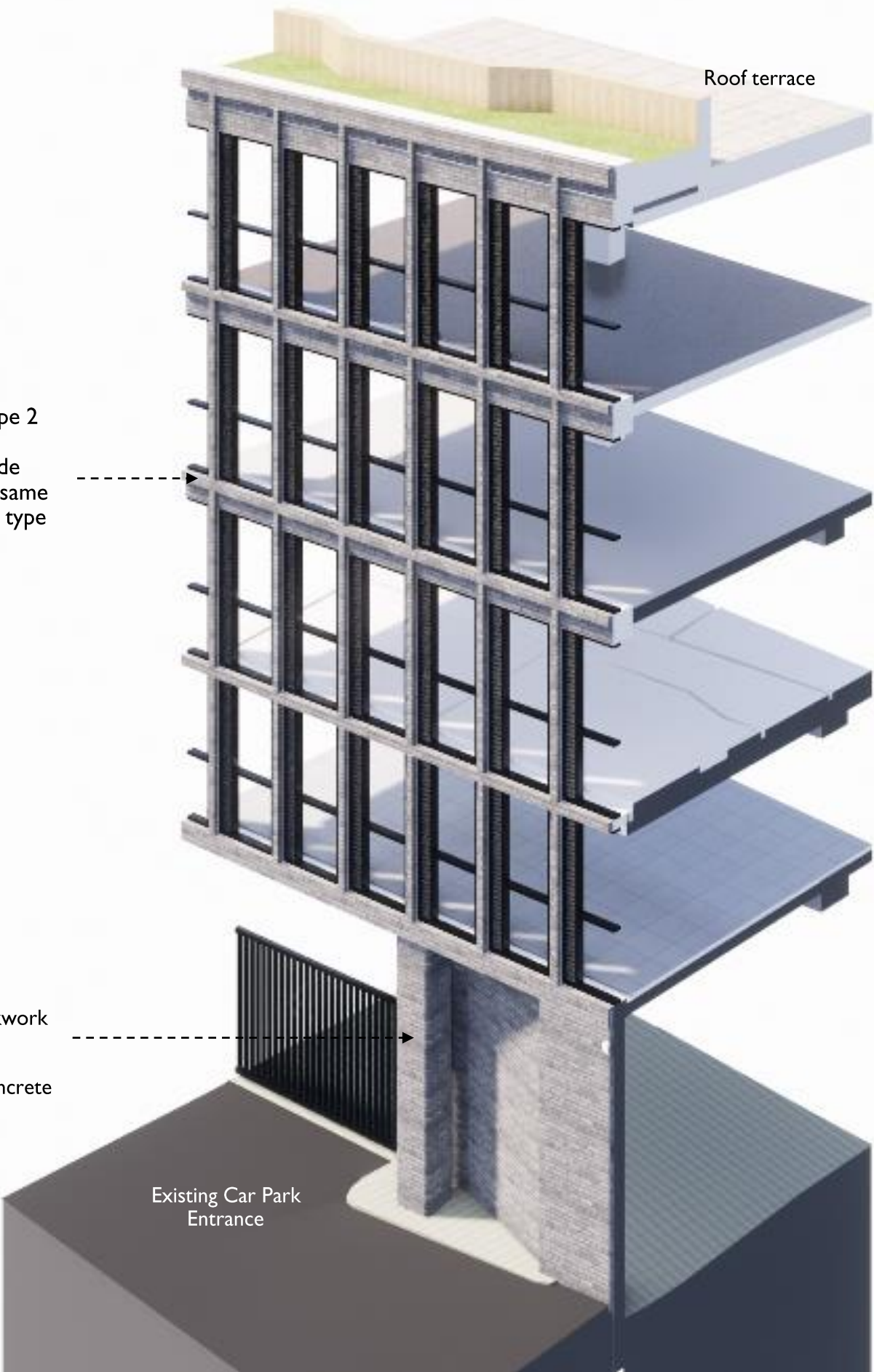
3D View of bay
