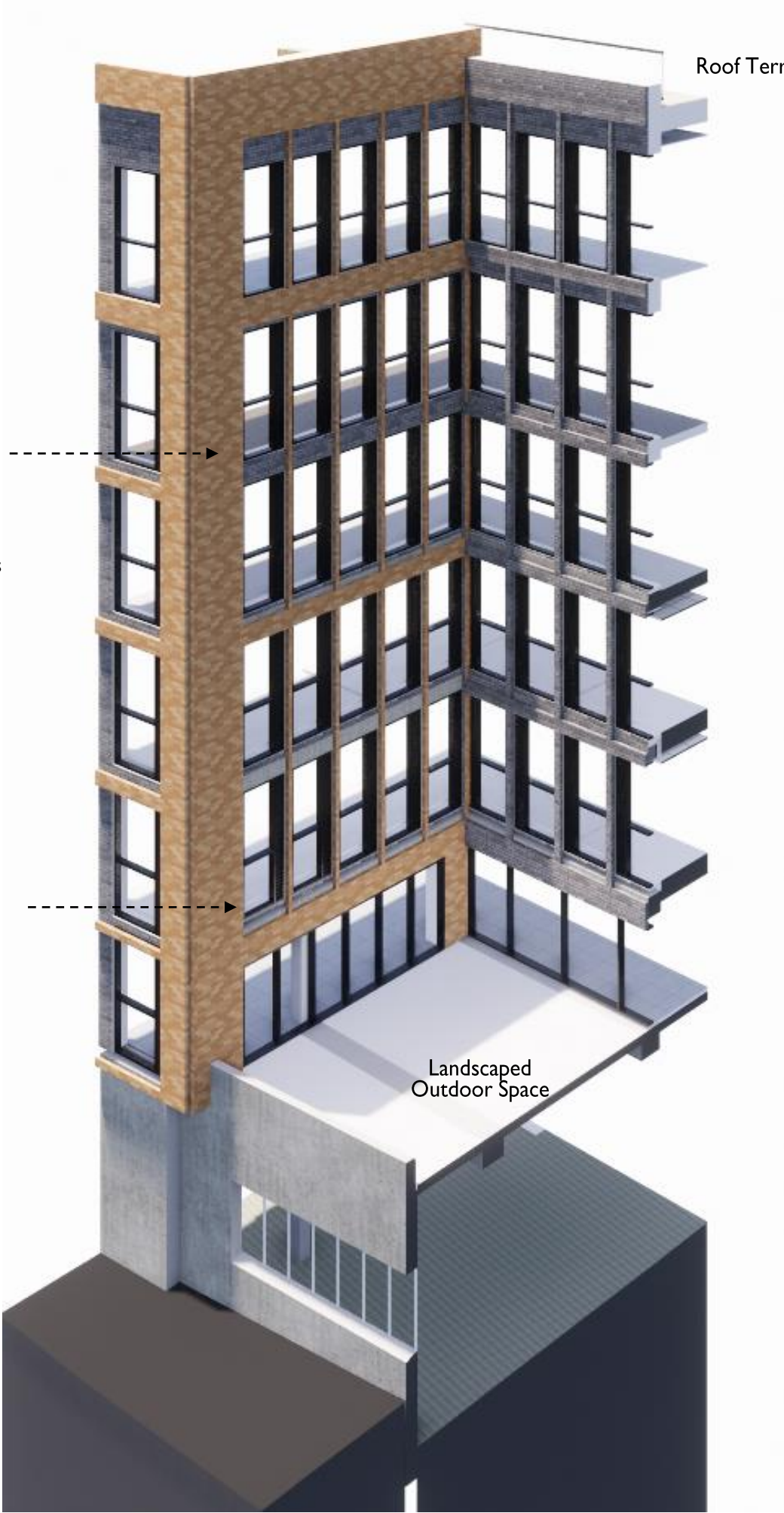
3D View of bay
