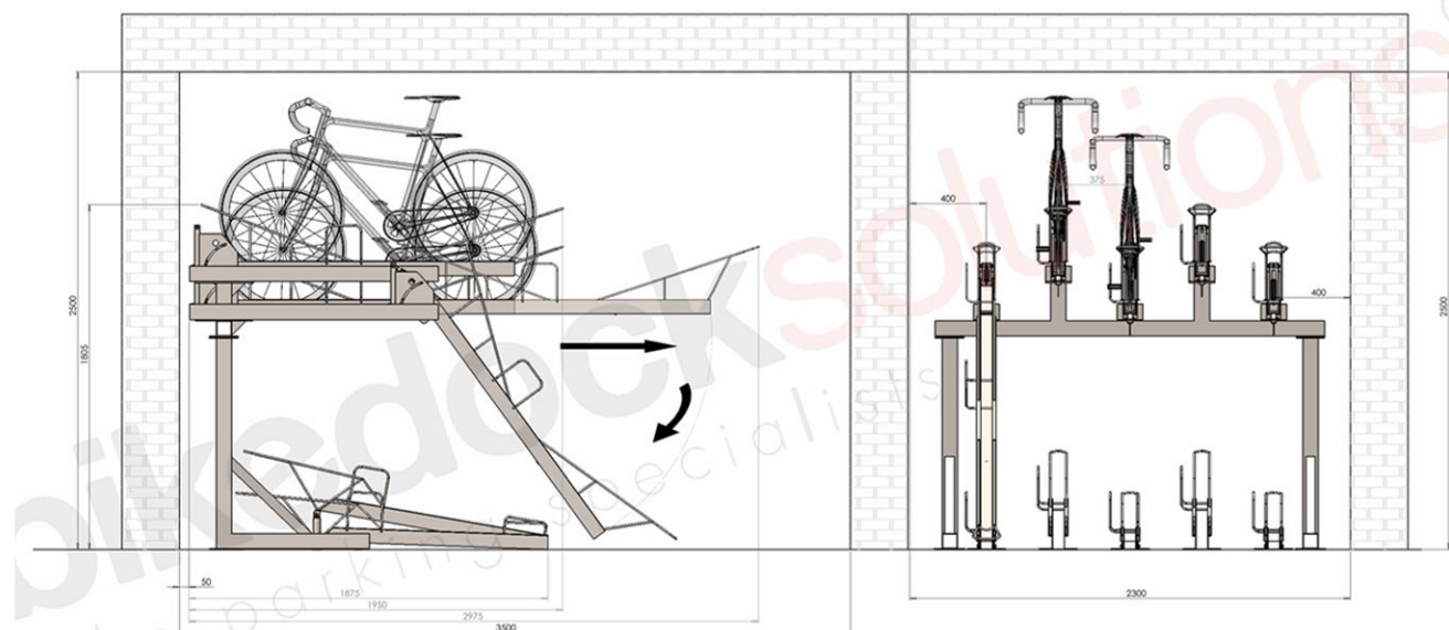
cycle store accommodates 3no. double tier cycle dock units and 2no. hoops
