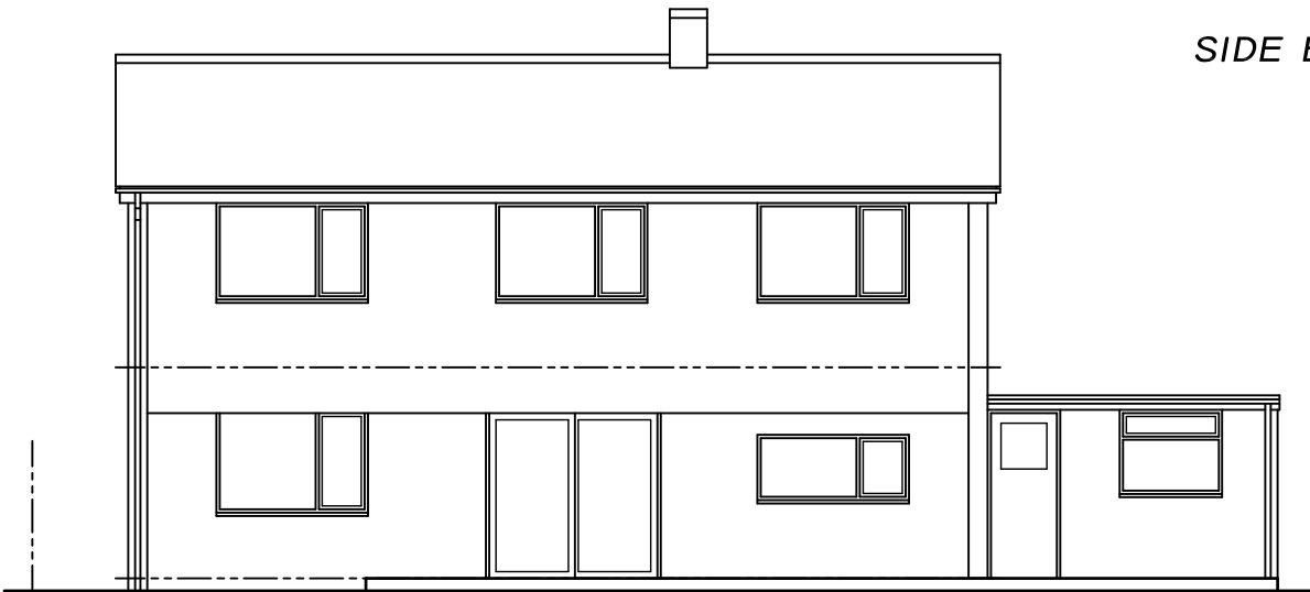
REAR ELEVATION
