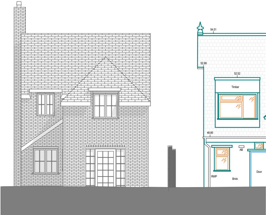
E-08 Proposed Rear Elevation cP 1:100
