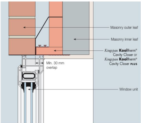
Figure 13 – Head Detail Incorporating Kingspan Kooltherm ® Cavity Closer
