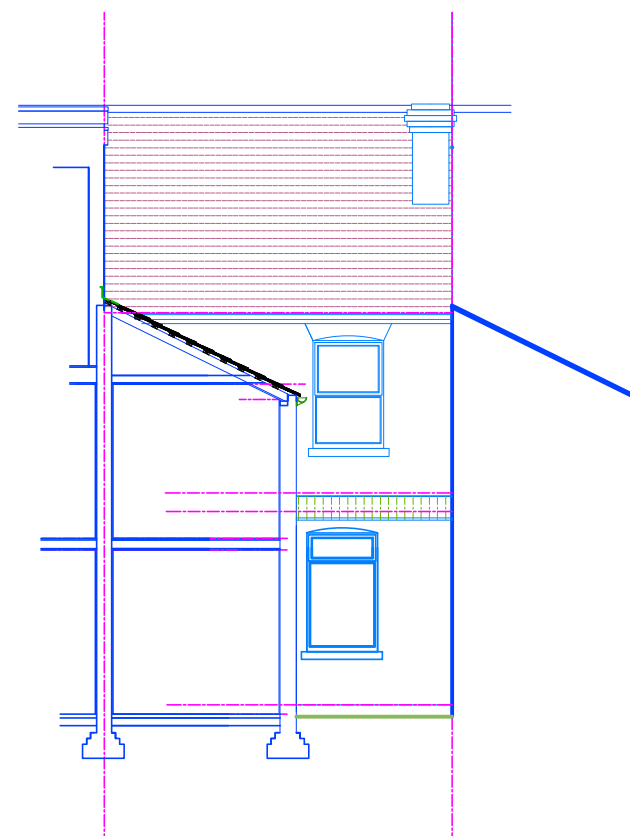
SECTION
