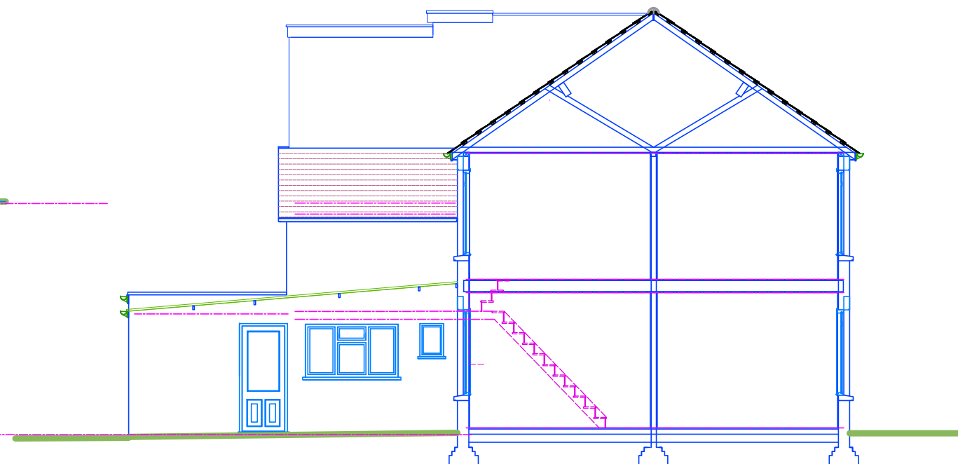
NORTH ELEVATION
