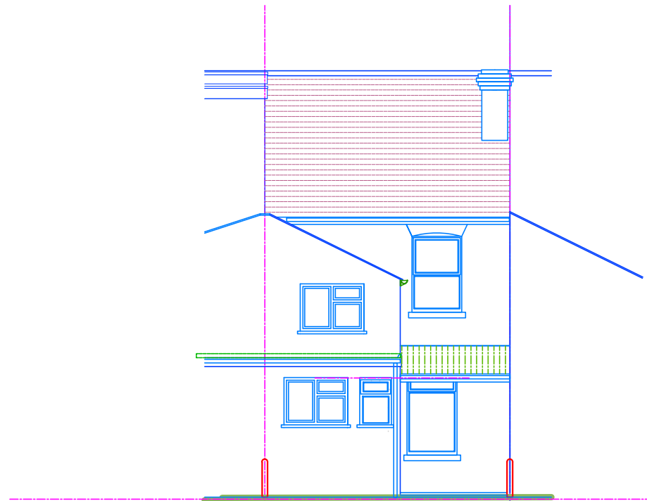
EAST ELEVATION
