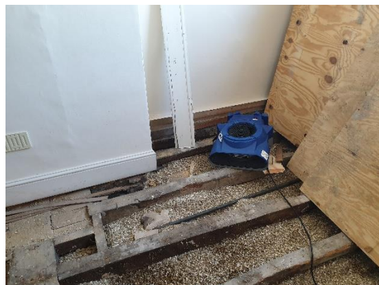
Plywood floor to be replaced to match existing
