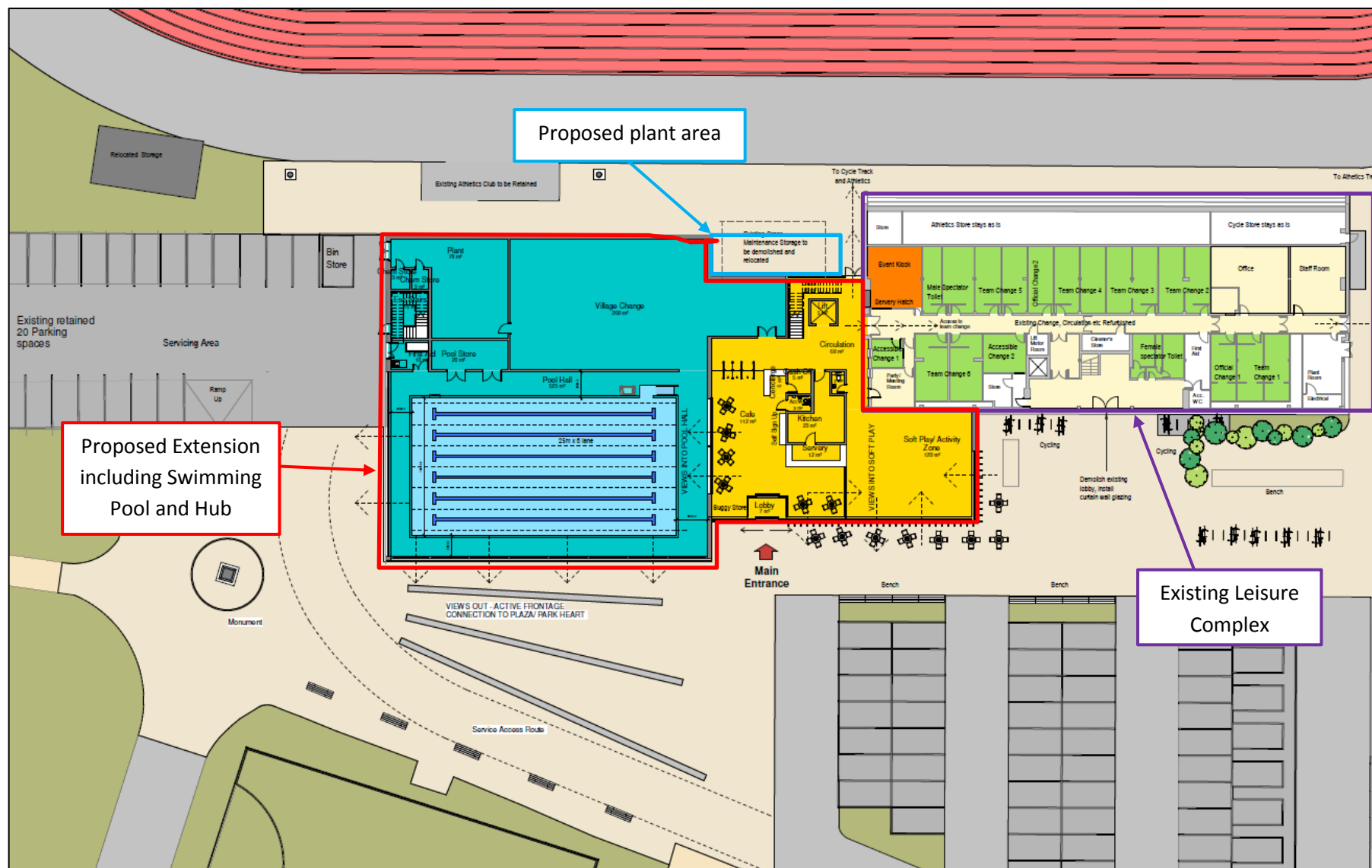
Figure 2.2: Proposed Site Layout Plan
