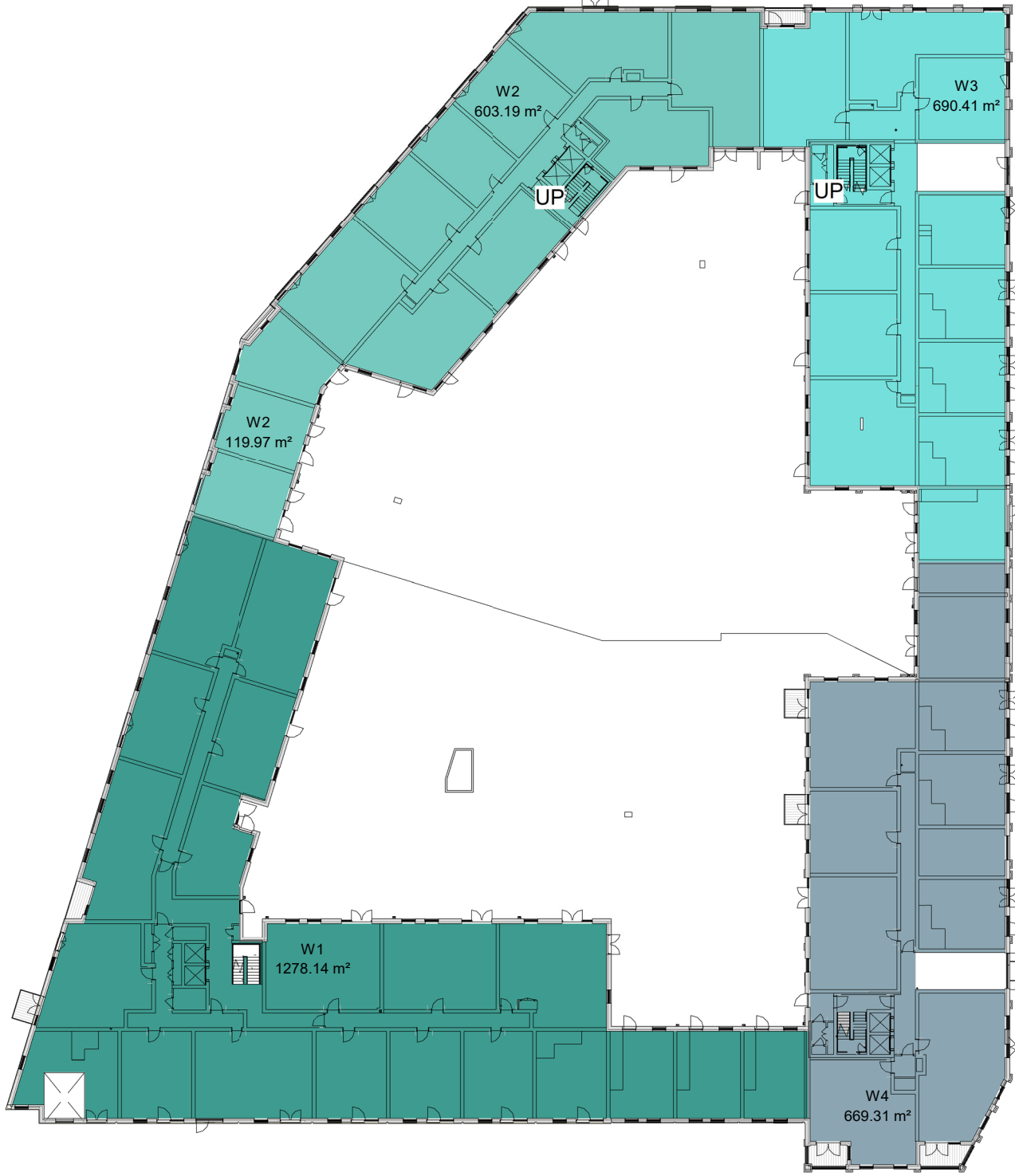
Level 1 and Level 2 1 : 500
