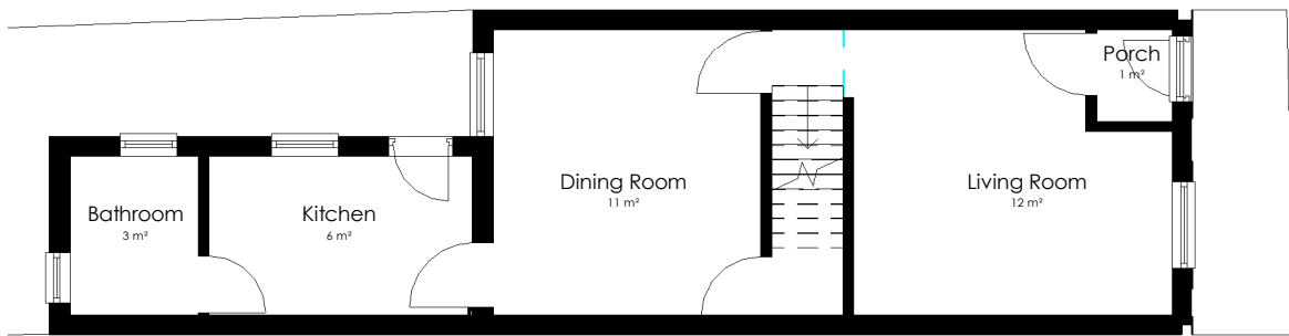
Existing Ground Floor 1 : 100
