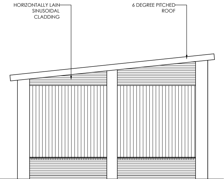
WEST ELEVATION
