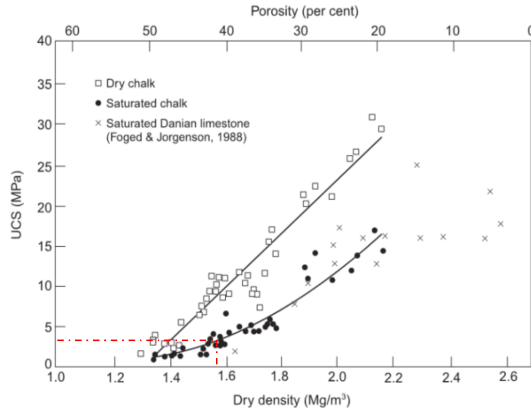
Figure 5.21: Relationship between unconfined compressive strength and intact dry density
