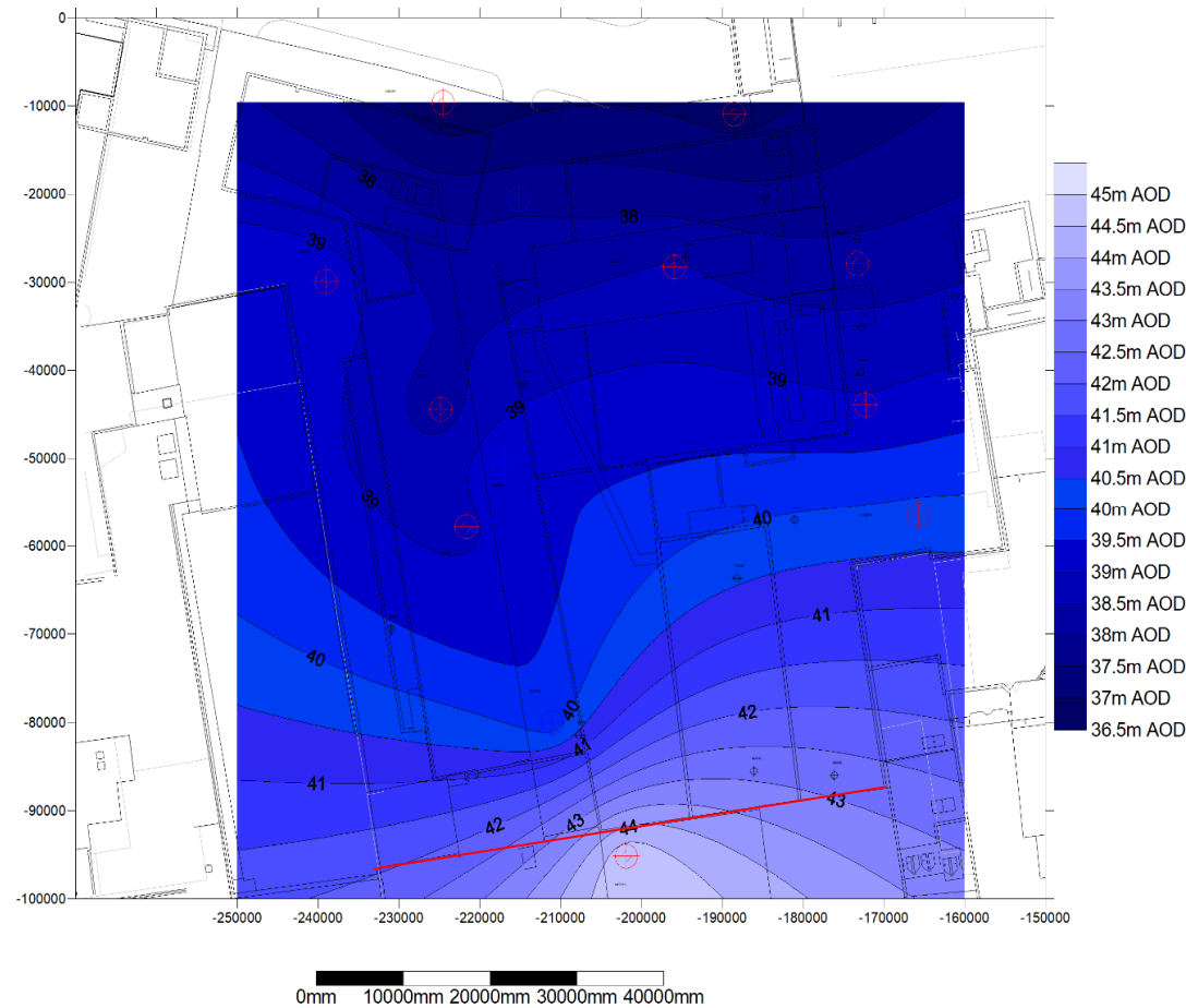
Figure 5.14 Contour Map showing the level of the Structureless Chalk across the site
