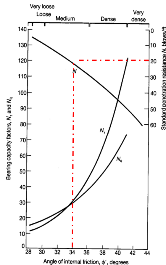
Figure 5.5 Relation between NSPT value and Angle of internal friction. Taken from CIRIA 143.
