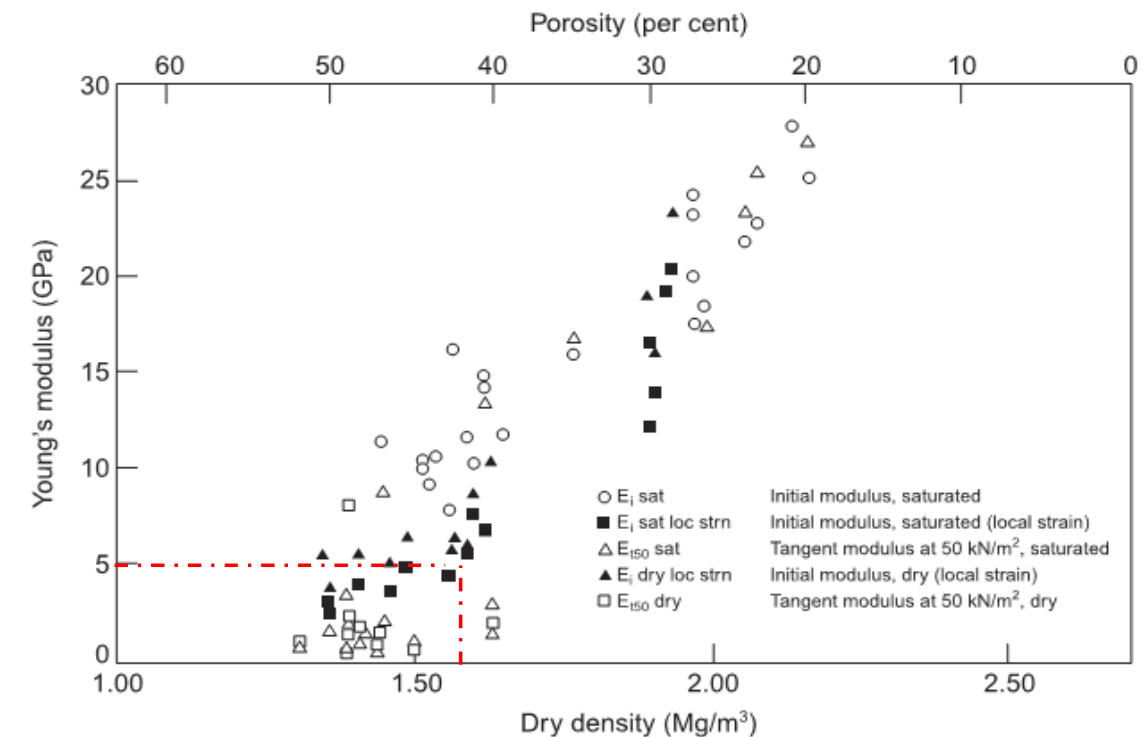
Figure 5.32 Relationship between dry density and porosity to Intact Youngs Modulus (Matthews and Clayton 1993). CIRIA 574.
