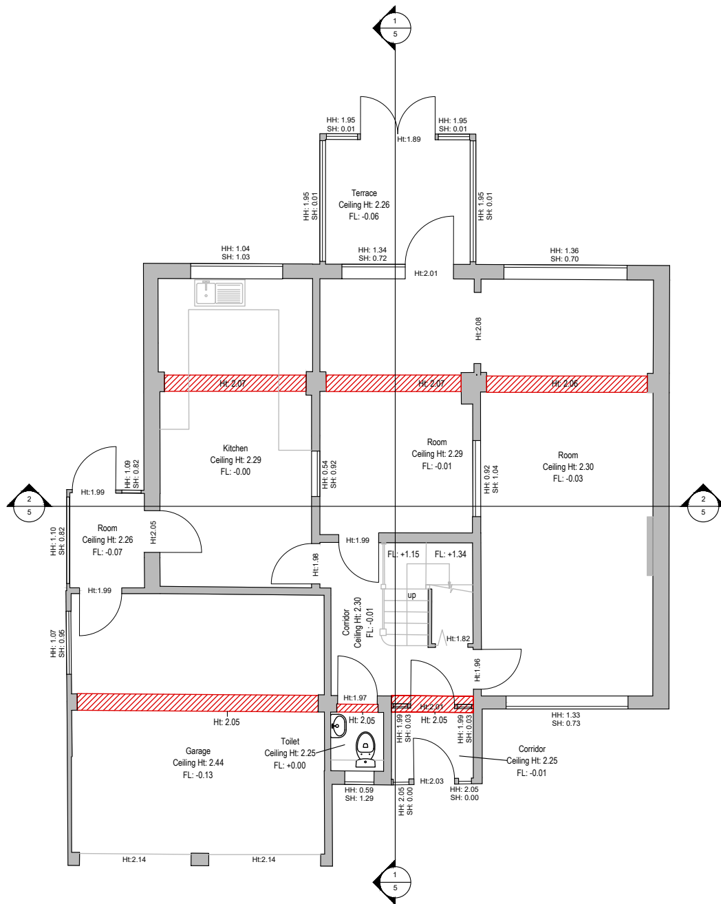
EXISTING GROUND FLOOR PLAN 1:100@A3
