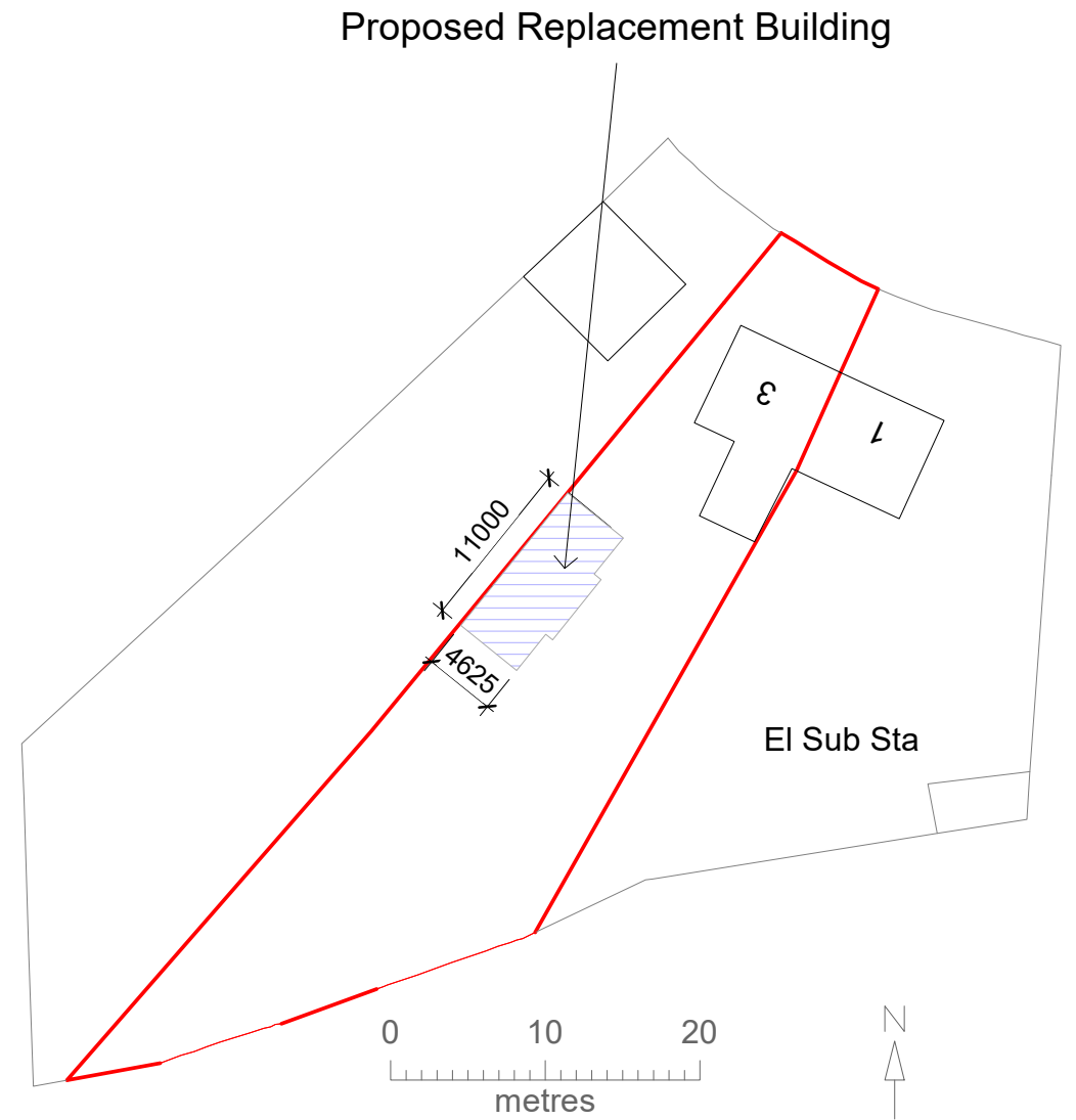
1 500 Proposed Site Plan 1 : 500
