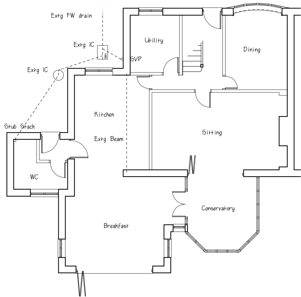
Extg GF Plan
