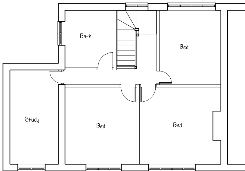
Extg FF Plan
