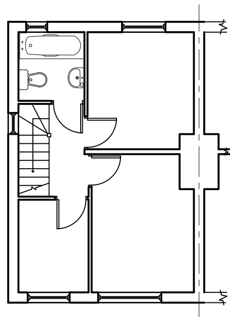
EXISTING 1ST FLOOR PLAN
