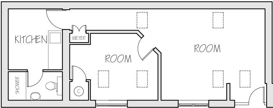
Ground Floor Plan (1:100)
